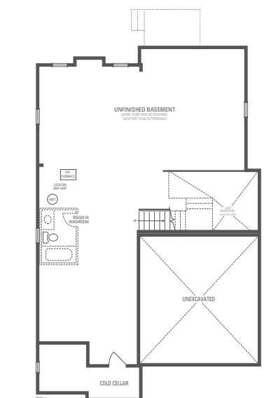
WALK-OUT BASEMENT (AVAILABLE ON SELECT LOTS)
